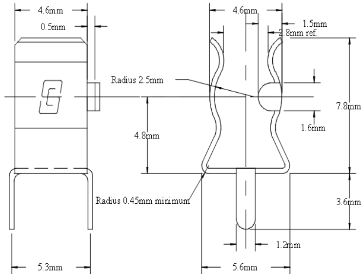
FC-53-11 5mm fuse clip with end stop and PCB lug, tin plated
