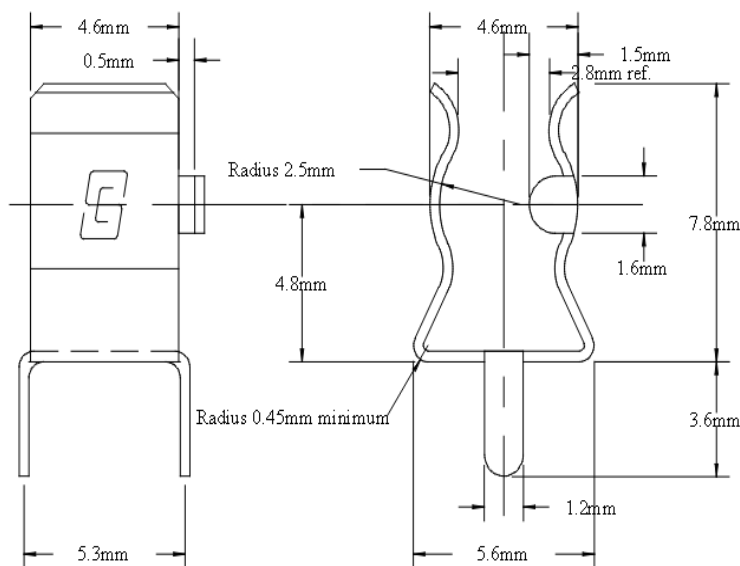
FC-53-12 5mm fuse clip with end stop and PCB lug, silver plated
